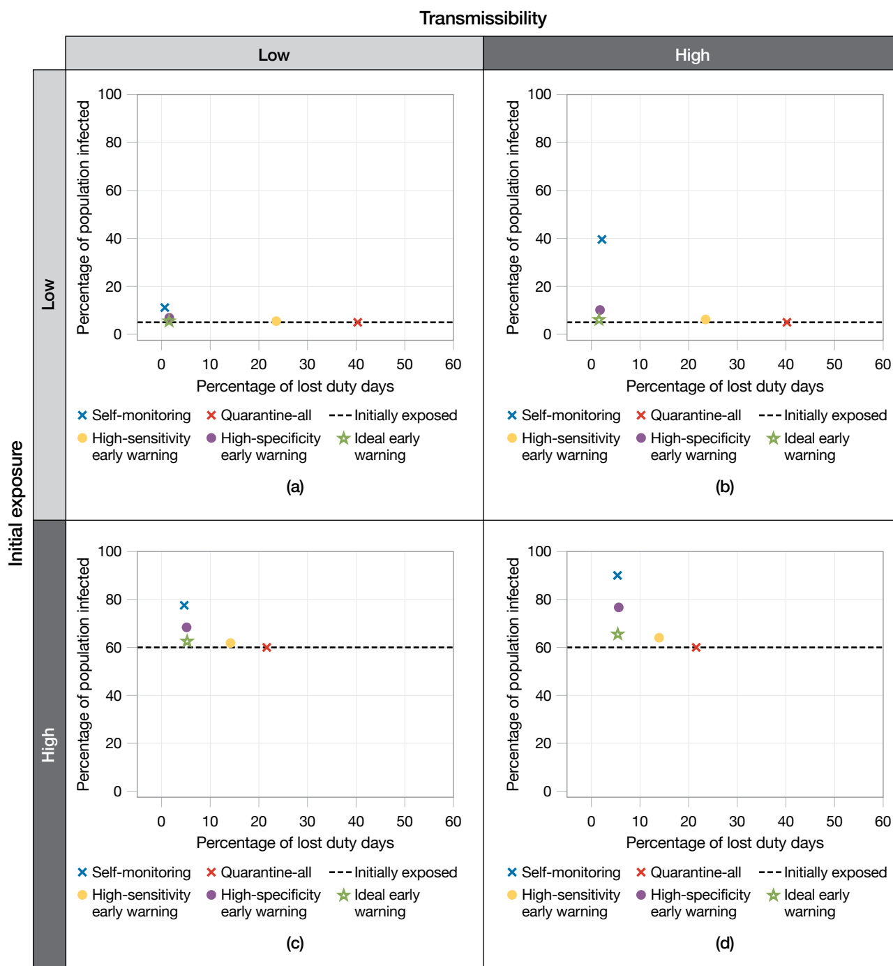
FIGURE 11. The trade space for the percentage of population infected versus percentage of lost duty days compares the augmented policies: self-monitoring, quarantine-all, and quarantine-on-alert with three levels of early warning performance (high sensitivity, high specificity, and ideal early warning). Four situations were considered: low-transmissibility pathogen with a low initial exposure (a), high-transmissibility pathogen with a low initial exposure (b), low-transmissibility pathogen with a high initial exposure (c), and high-transmissibility pathogen with a high initial exposure (d).
