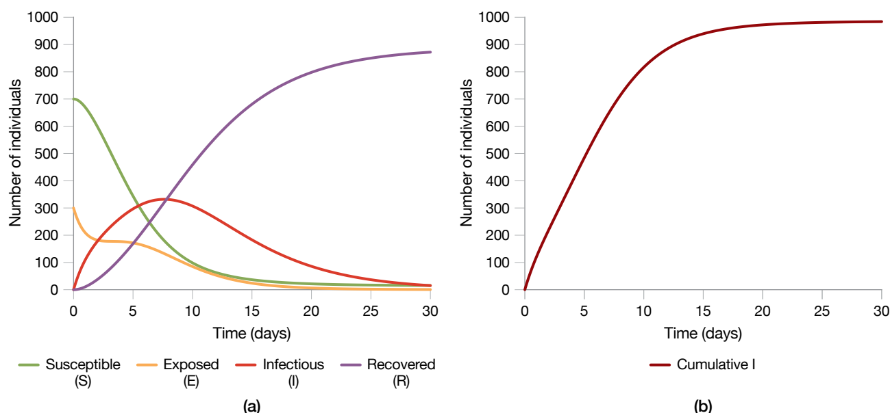
FIGURE 2. A numeric solution for the baseline SEIR model shows the population of each compartment versus time (a), which indicates that for an initial exposure of 300 individuals, nearly the entire population will eventually fall ill; the cumulative number of infections (Cumulative I) versus time is shown in (b).
