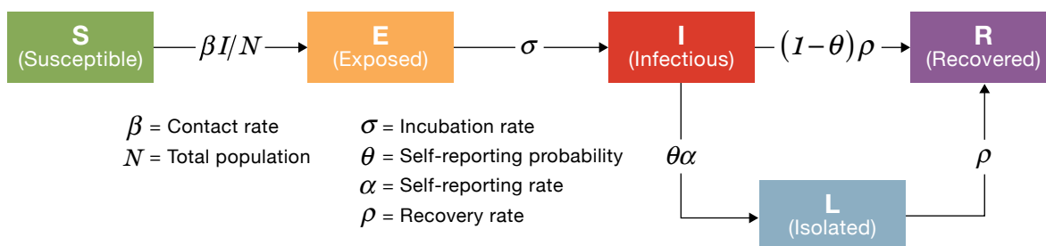
FIGURE 3. The model diagram for a self-monitoring and self-reporting policy includes an additional compartment ( L ) for individuals who are isolated after developing symptoms. Note that fatalities are left out for simplicity.
