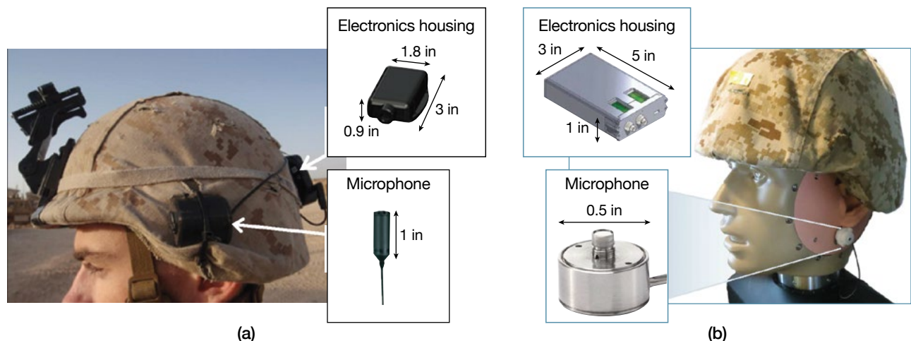
FIGURE 3. The first- (a) and second-generation (b) Lincoln Laboratory noise dosimeters are depicted.
